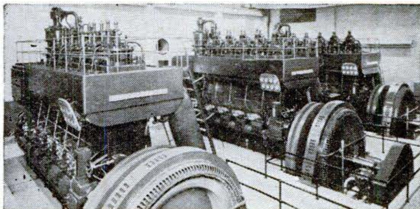
A typical modern Diesel plant.
